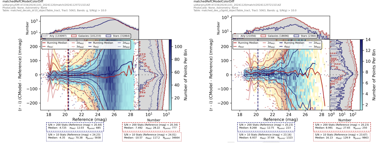
Figure 50: Difference between r - i CModel colors and DECaLS/DES-Y3G catalog values in ECDFS.
