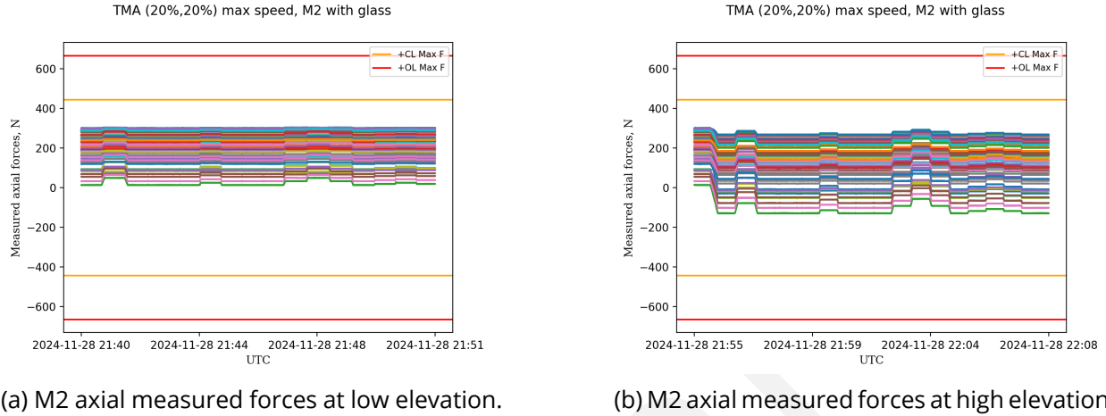
Figure 9: M2 axial measured forces during the slews at different elevations.
