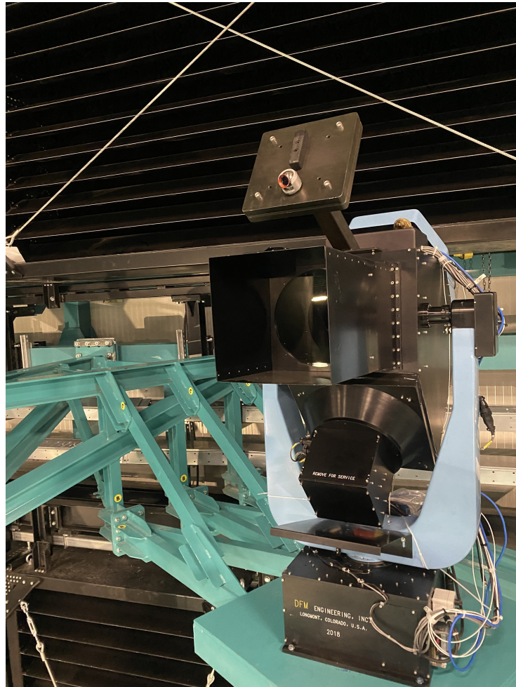
FIGURE 1: Image of the CBP, which was installed on the dome on November 22.
