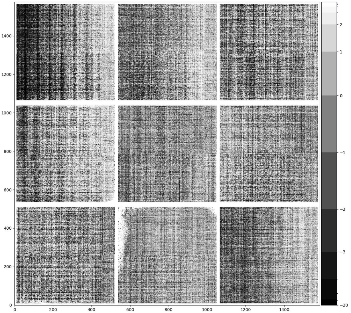
FIGURE 3: The phosphorescence seen in R22_S01, shown here in a dark exposure taken after a series of twilight flats (exposure=2024112000065). This material absorbs light at bluer wavelengths and re-emits that energy over a wide range of wavelengths.
