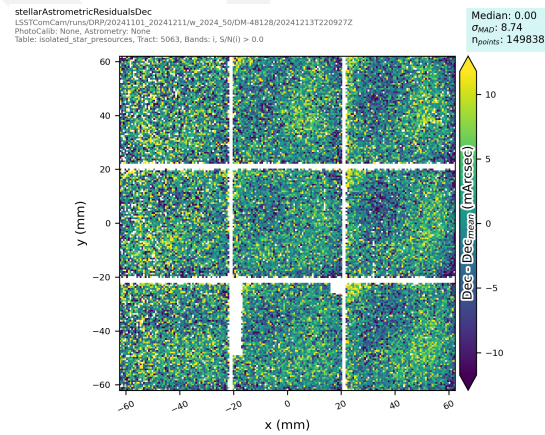
FIGURE 8: Declination residuals projected in Focal plane coordinate for a given tract. Some structure looks to be present in focal plane coordinates, which will be taken into account with GBDES.
