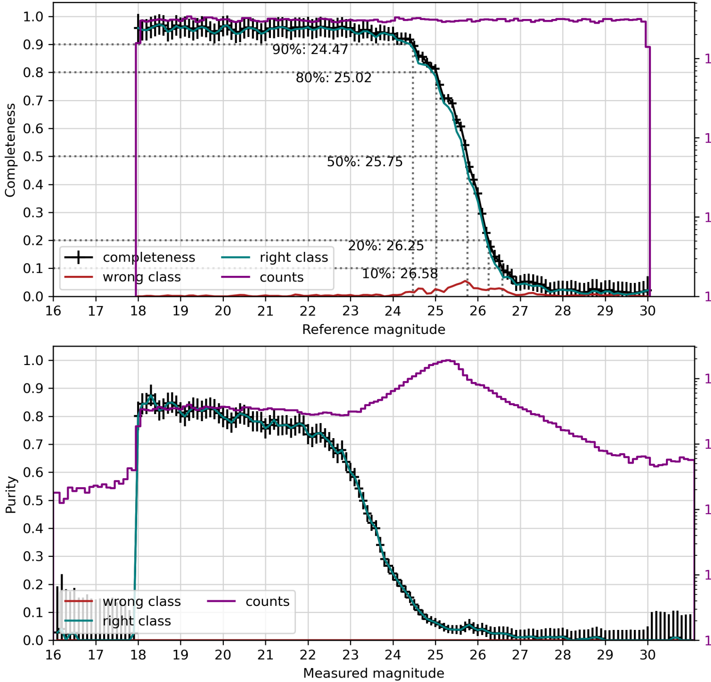
FIGURE 7: SSI based measurements of completeness and purity in the i-band.
