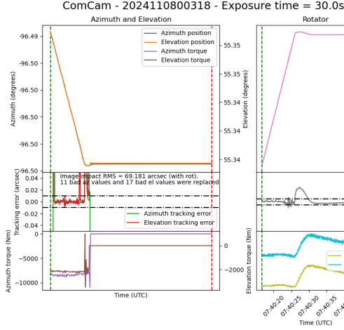
Figure 21: Exposure with an unusually large amount of mount motion image degradation.
