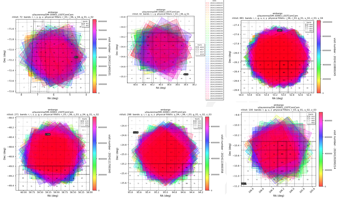
Figure 1: Sky coverage for six ComCam Deep Drilling Fields. First Row (left to right): 47 Tuc, Fornax dSph, ECDFS. Second Row (left to right): EDFs, RubinSV 95 -25, Seagull.
