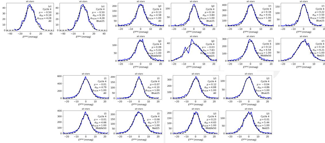
Figure 40: Photometric repeatability for stars in the ugriz bands.
