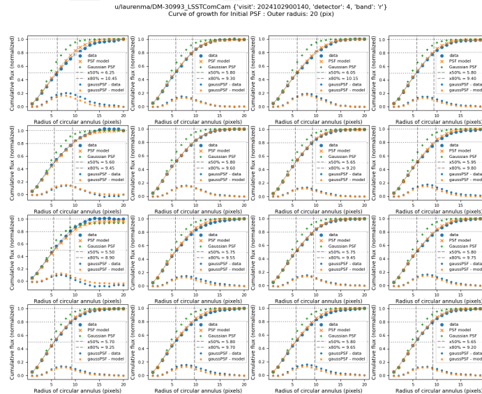
Figure 23: Growth curves of the PSF compared to its model (PSFex here) in the early data taken with ComCam.
