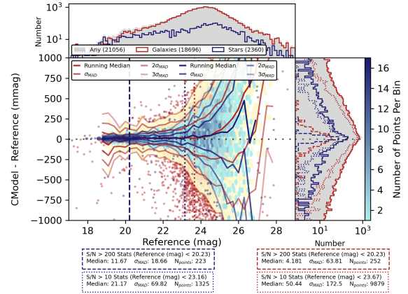
Figure 48: Difference between g-band CModel magnitudes and DECaLS/DES-Y3G catalog values in ECDFS.
