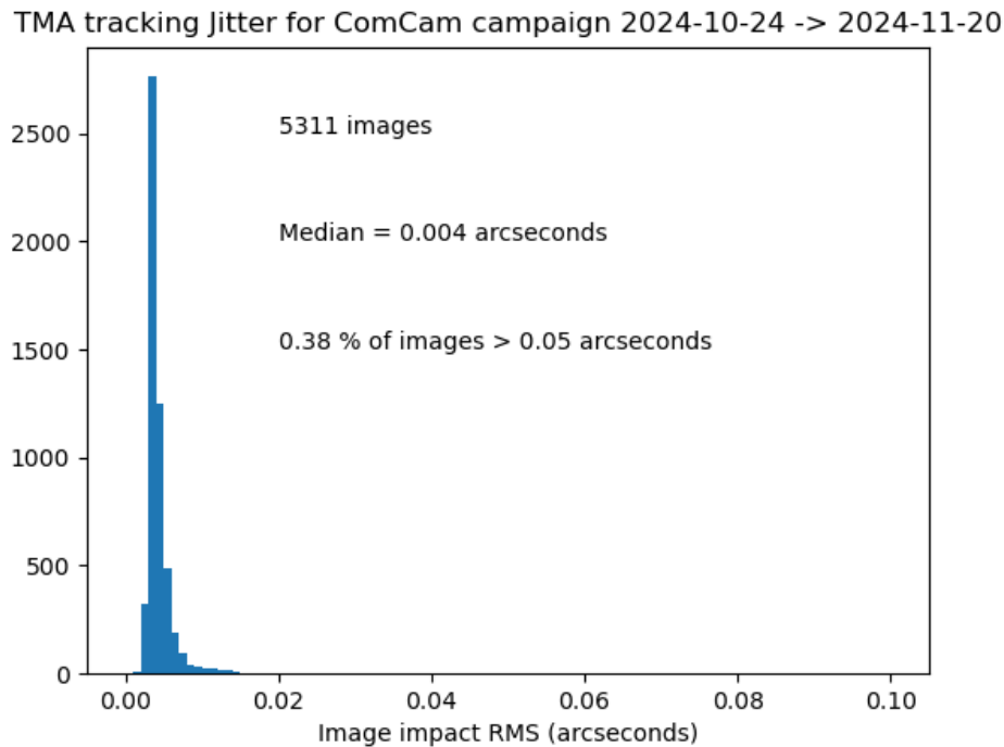
Figure 20: Total TMA tracking jitter for all exposures from October 24 to November 20.
