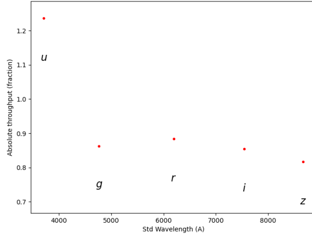
Figure 42: Absolute throughput derived per band, relative to naive expectations.
