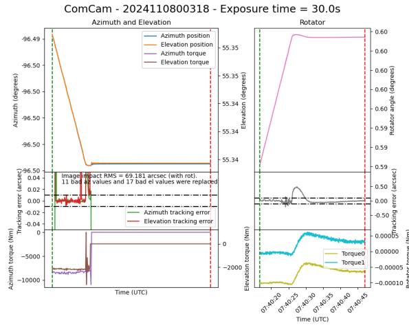
Figure 21: Exposure with an unusually large amount of mount motion image degradation.
