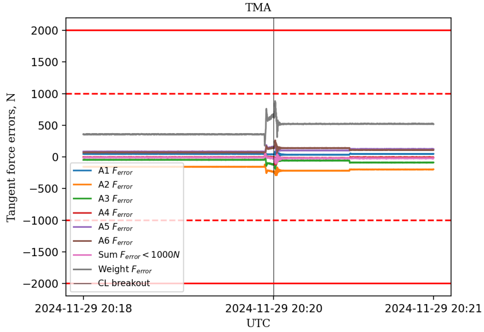
Figure 14: M2 tangential force errors during the closed-loop break-out test.
