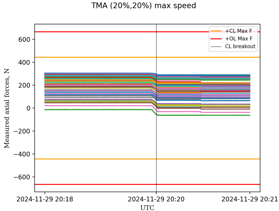
Figure 12: M2 axial measured forces during the closed-loop break-out test.
