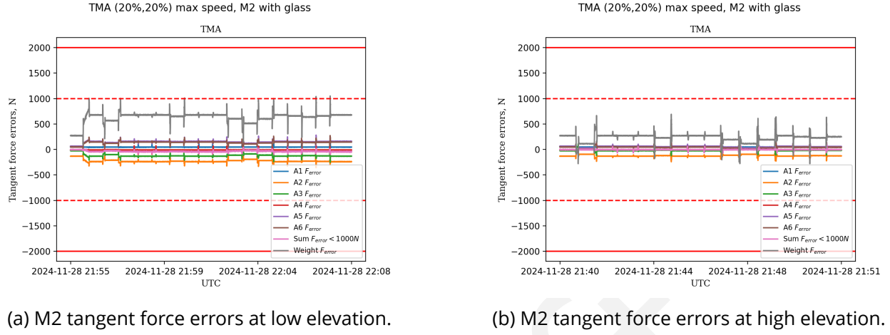
Figure 11: M2 tangent force errors during the slews at different elevations.
