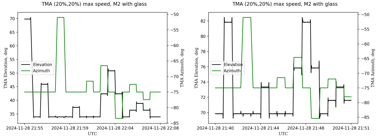
Figure 6: TMA Short and Long slews at El = 34^\circ (left) and El = 70^\circ (right).
